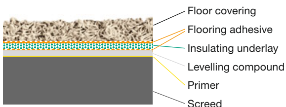
Floor construction
